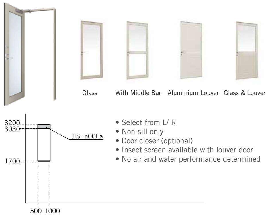
In-Swing Door (Single)
