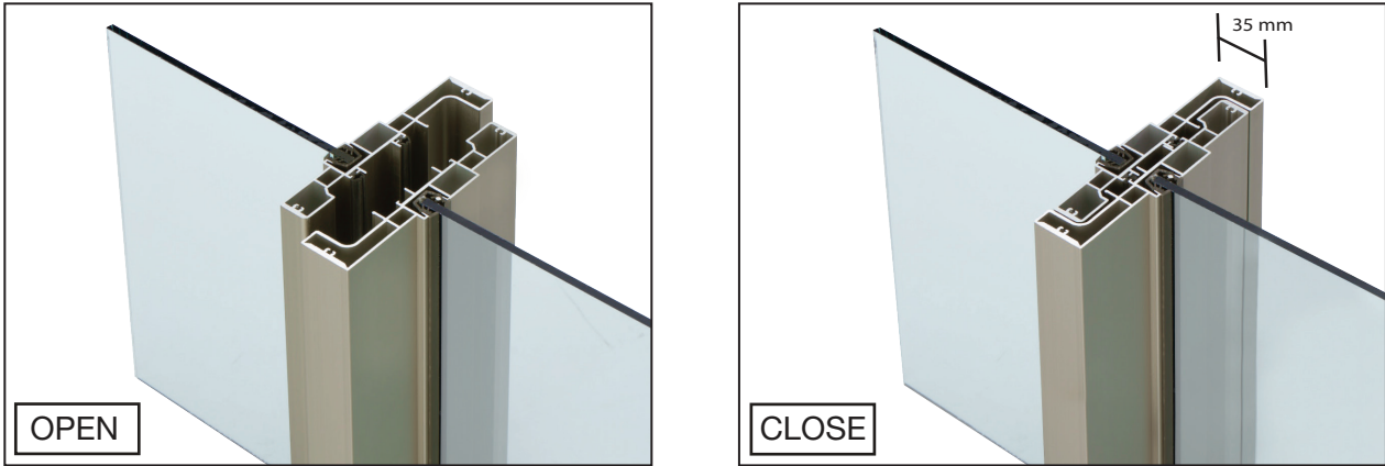
Overlapping meeting stile (4 Panels Sliding)
