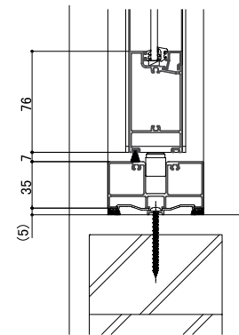
<Vertical section: Flat sill>
