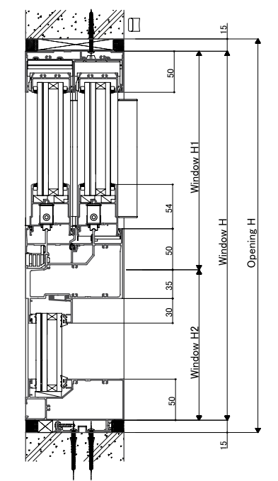
<Vertical section: Sliding/Fix A-A'>
