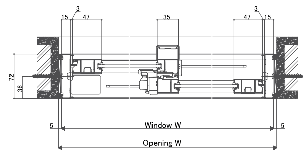
<Horizontal section: 2 panels sliding window>
