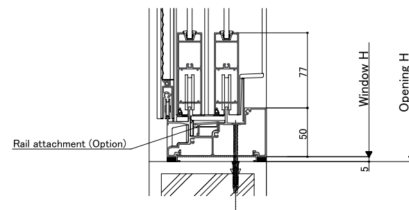
<Sill detail: With rail attachment>
