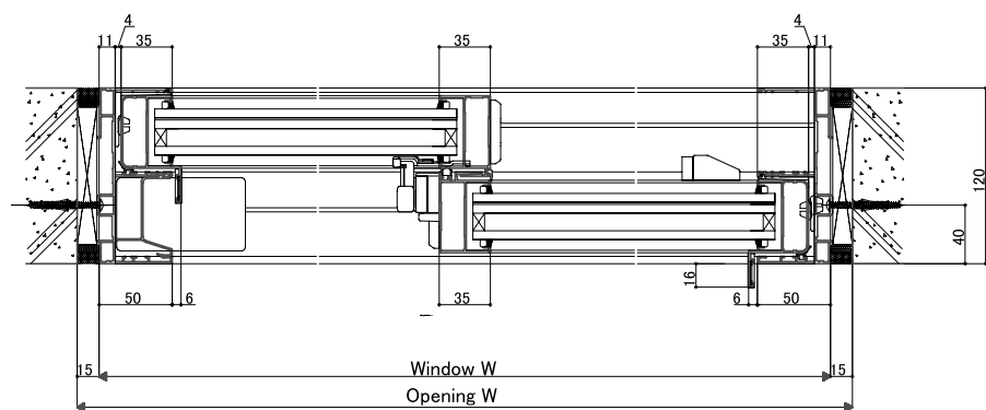
<Horizontal section: 2panels sliding window >
