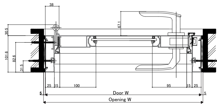
<Horizontal section: Single out-swing door>
