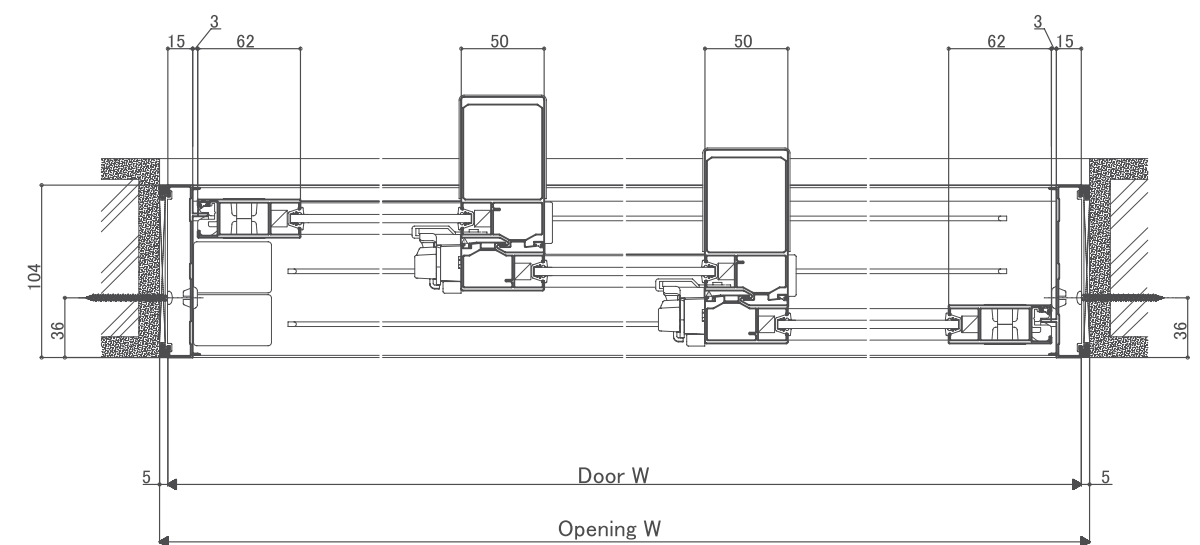
<Horizontal section: 3 panels sliding door>
