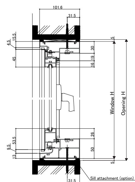
<Vertical section: Double casement window>
