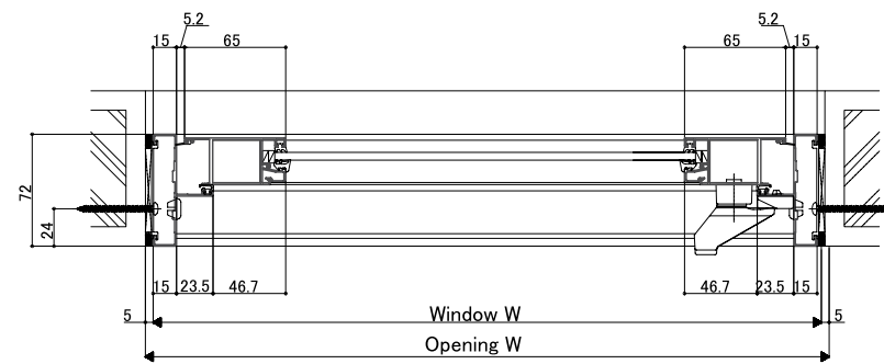
<Horizontal section: Casement (single lock)>
