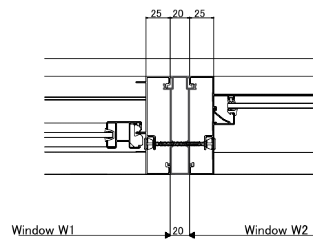
<Horizontal section: Mullion>
