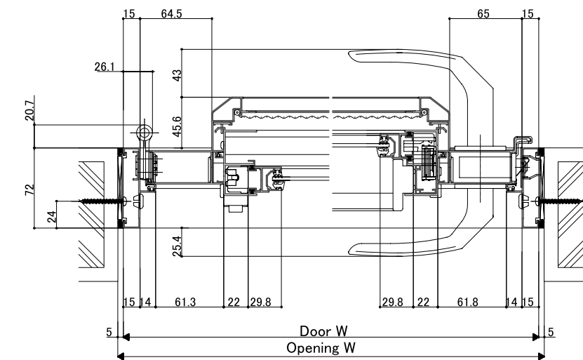
<Horizontal section: Ventilation Door>
