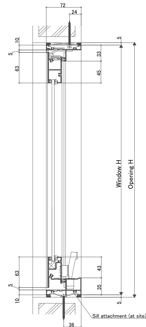
<Vertical section: Awning (single lock)>
