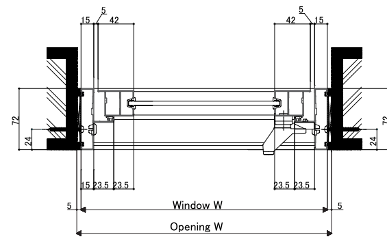
<Horizontal section: Casement window>
