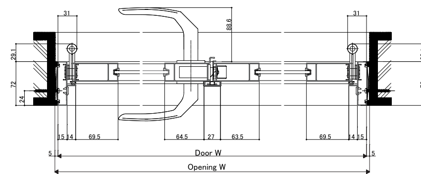
<Horizontal section: Double out-swing door>
