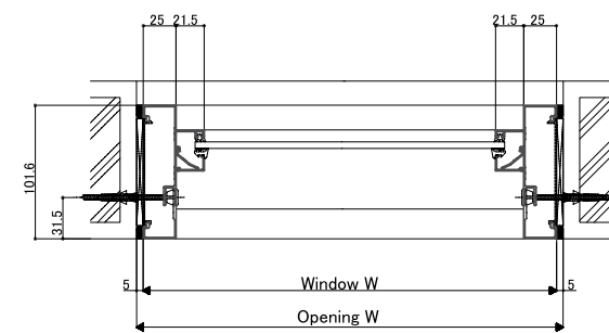
<Horizontal section: Single fix window>
