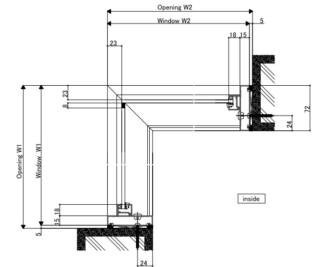
<Horizontal section: Outward fix window>
