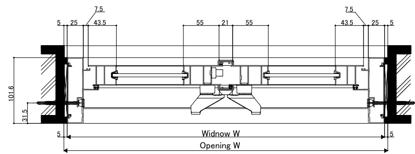
<Horizontal section: Double casement window>
