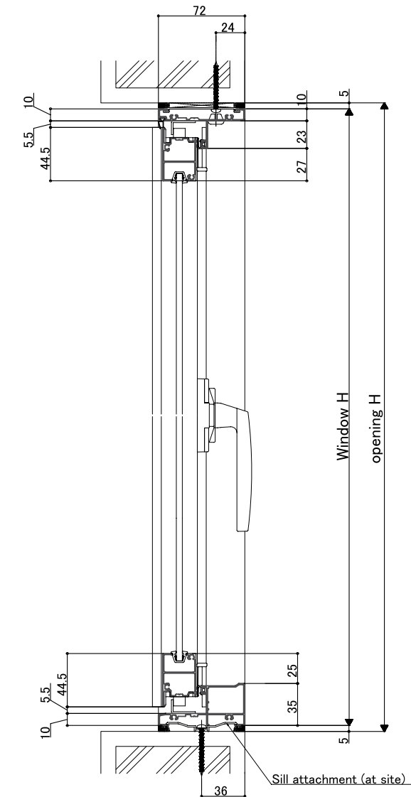
<Vertical section: Double casement window>
