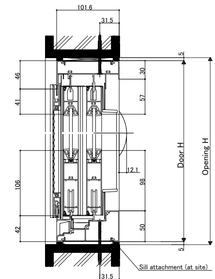
<Vertical section: 4 & SFS 3 panels sliding door>
