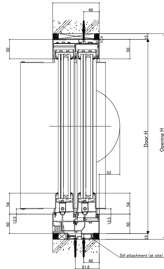
<Vertical section: 2 panels sliding door>
