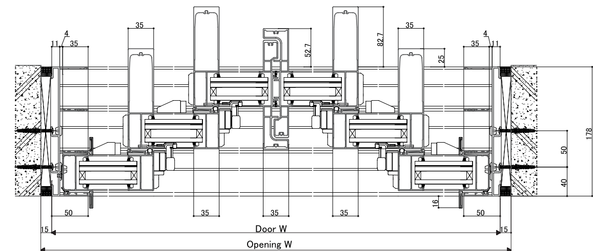
<Horizontal section: 6 panels sliding door (larger) >
