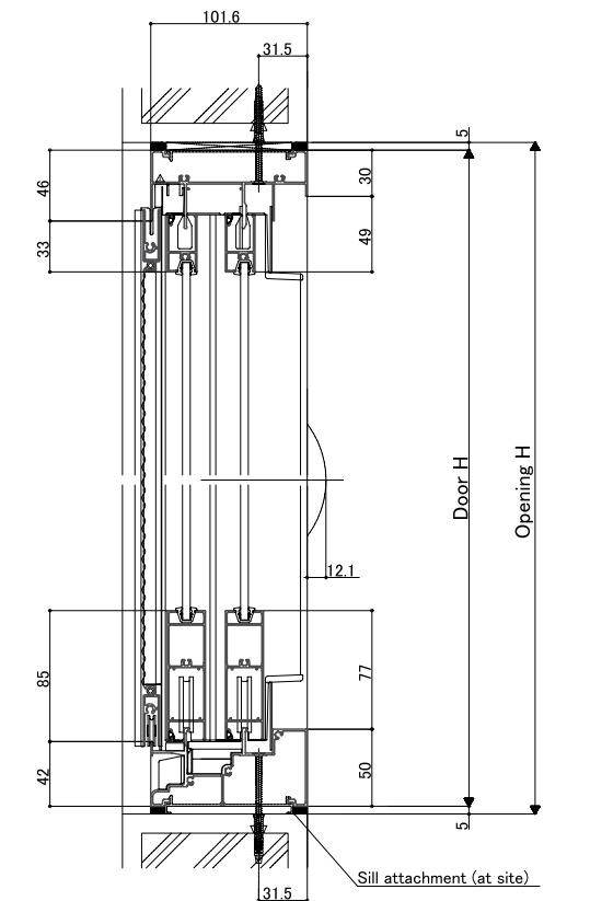
<Vertical section: 2 panels sliding door>
