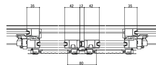
<Horizontal section: 4 panels sliding window>
