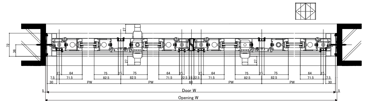
<Horizontal section: Center open folding door>
