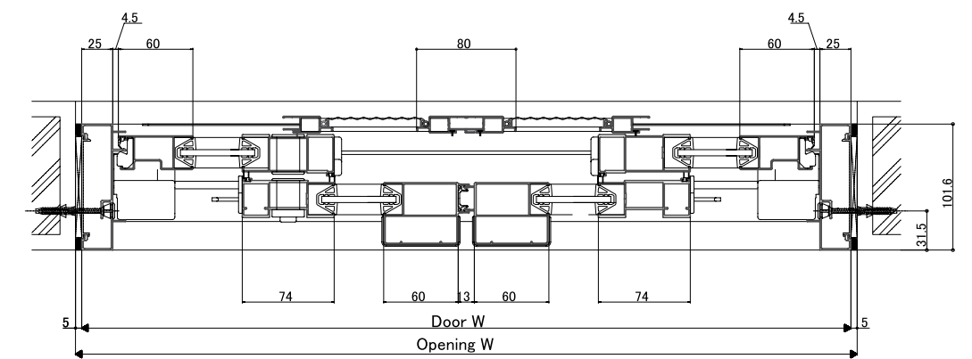
<Horizontal section: 4 panels sliding entrance door>
