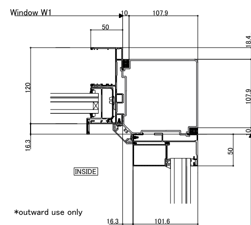
<Corner mullion with sliding window>
