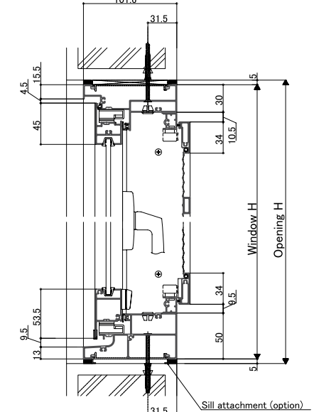
<Vertical section: Casement with screen>
