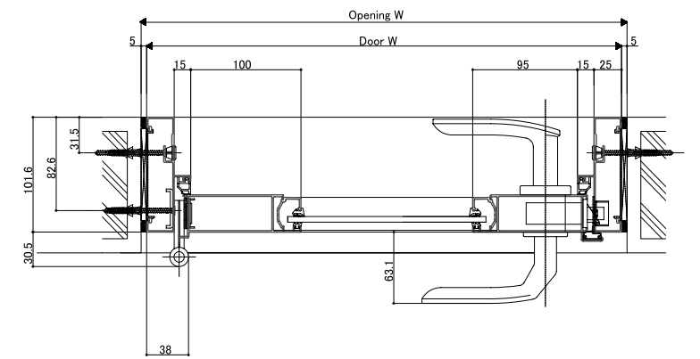
<Horizontal section: Single in-swing door >
