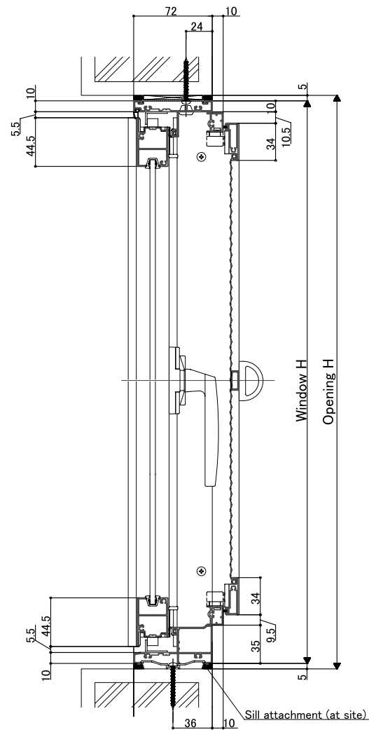
<Vertical section: Double casement with screen>
