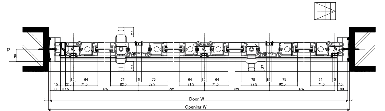
<Horizontal section: One way open folding door>
