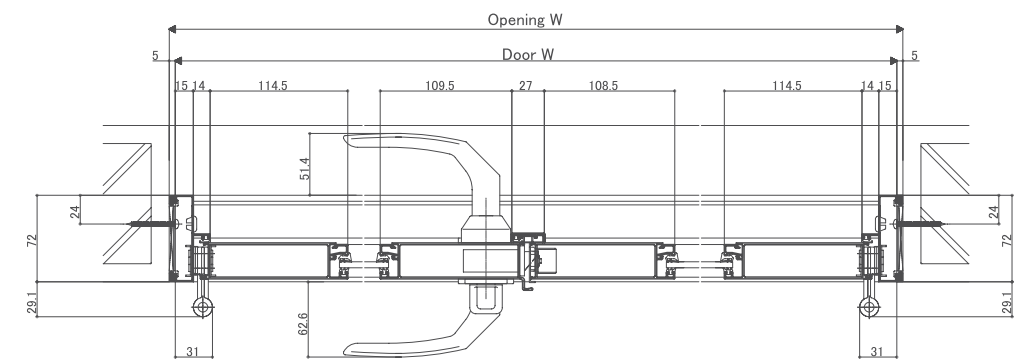
<Horizontal section: Double in-swing door>
