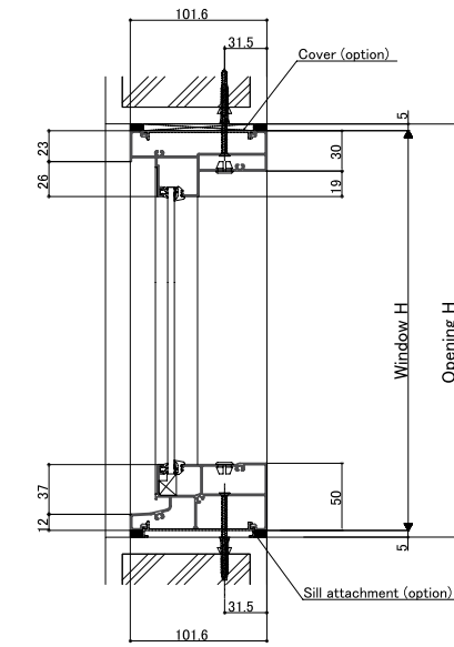
<Vertical section: Single and corner fix window>
