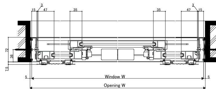
<Horizontal section: SFS 3 panels sliding window>
