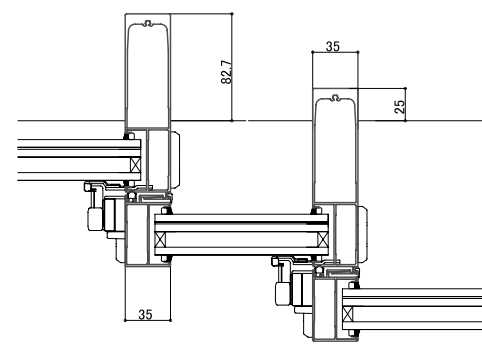
<Stile detail: In case of largest openings >
