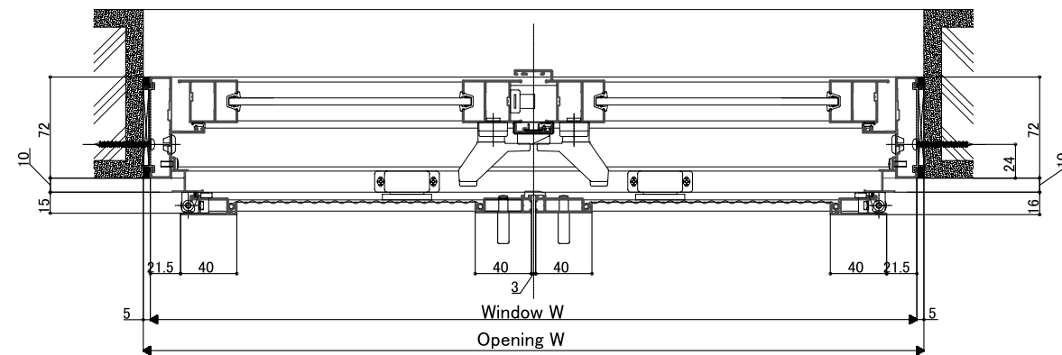
<Horizontal section: Double casement with screen>
