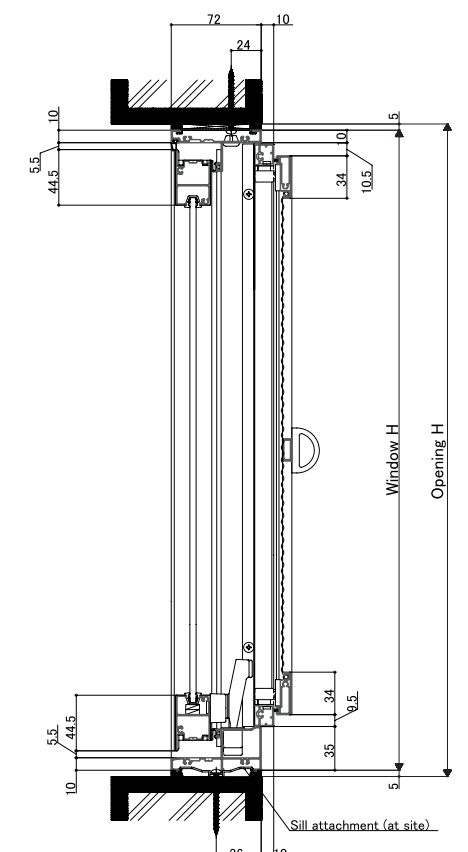
<Vertical section: Awning with screen>
