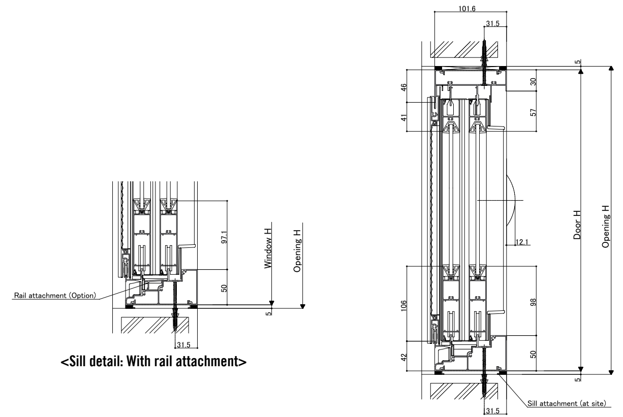
<Vertical section: 4 panels sliding entrance door>
