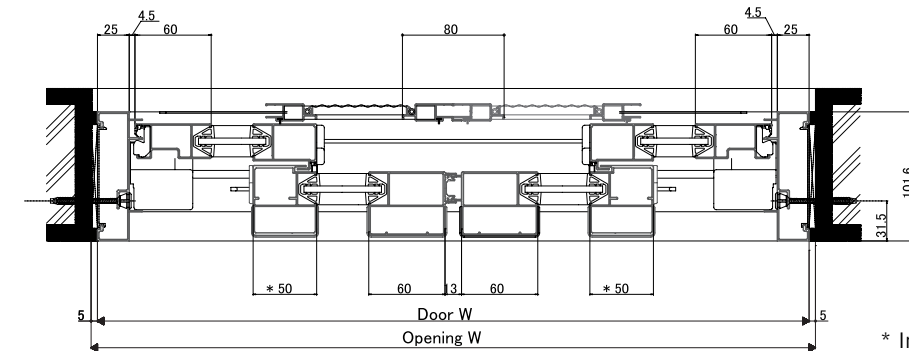
<Horizontal section: 4 panels sliding door>
