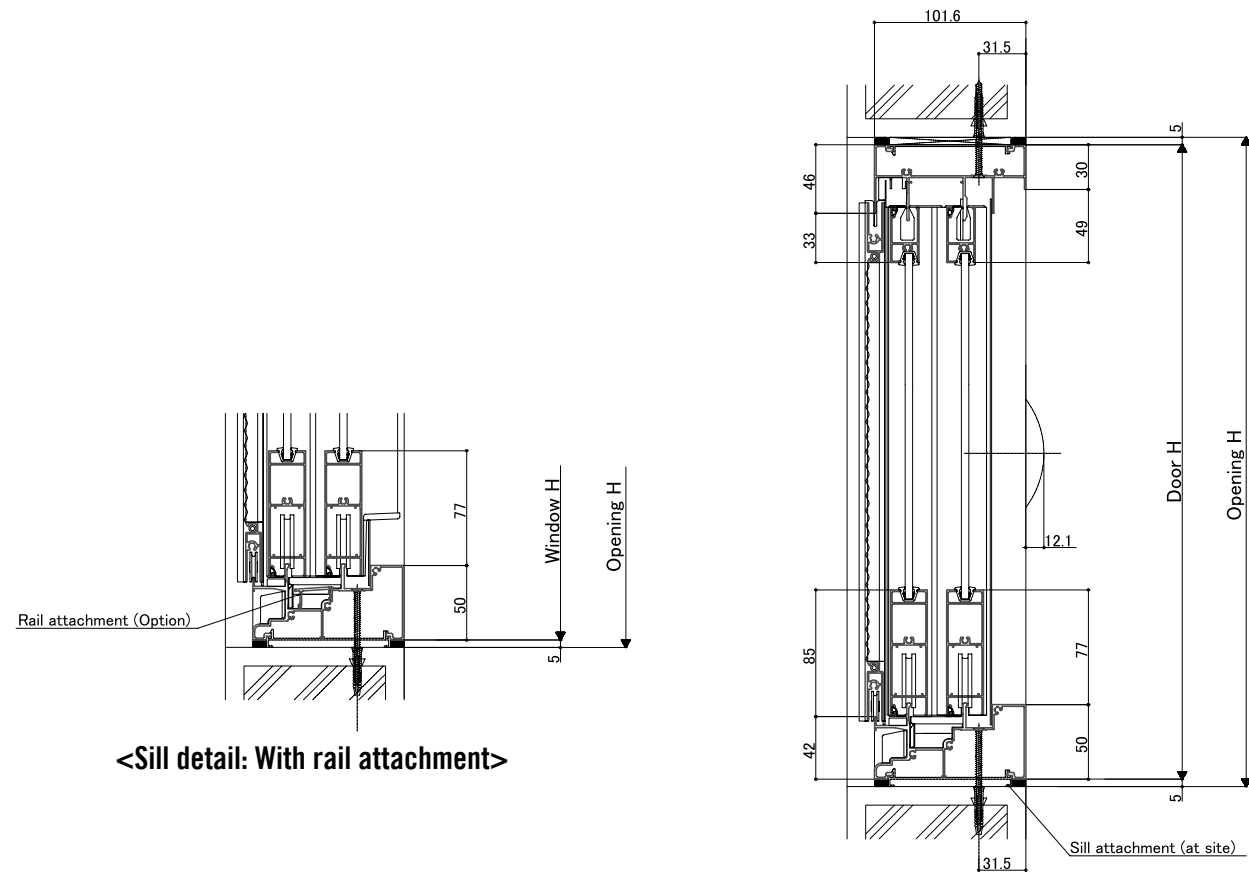
<Vertical section: 2 panels sliding entrance door>
