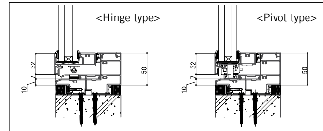
<Sill detail>
