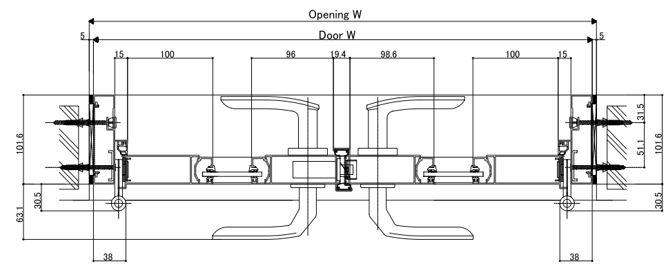
<Horizontal section: Double in-swing door>
