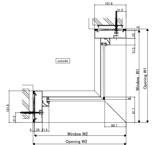
<Horizontal section: Inward fix window>
