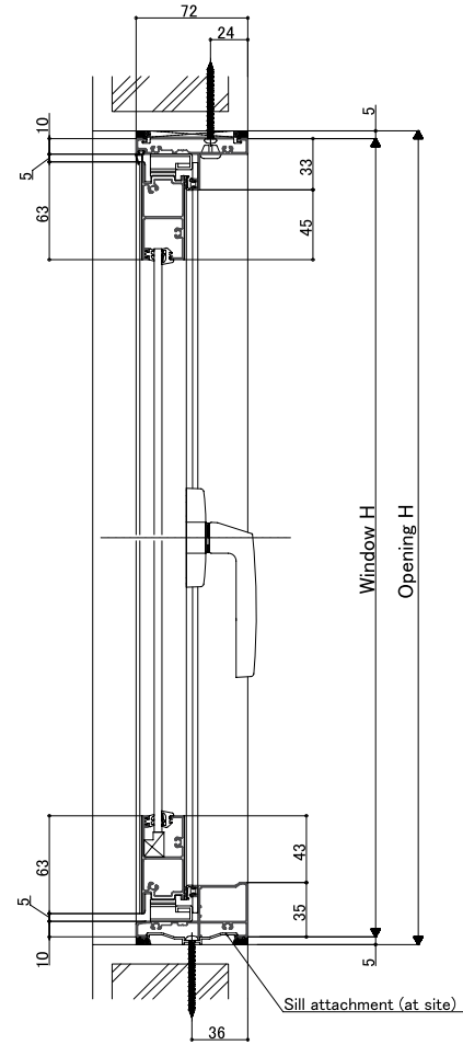
<Vertical section: Casement (single lock)>
