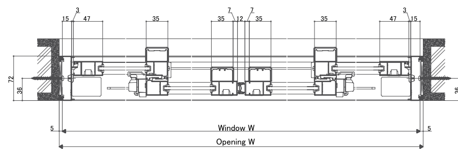
<Horizontal section: 4 panels sliding window>
