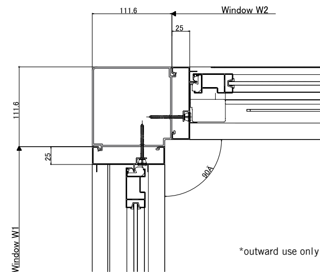
<Horizontal section: Corner mullion>
