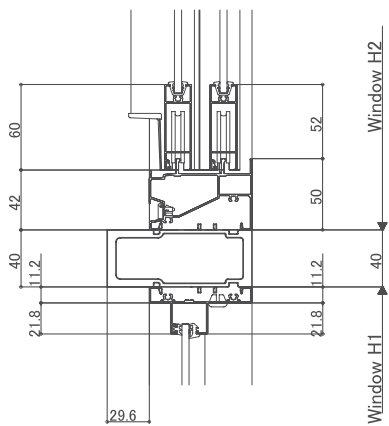
<Transom (Large)>
