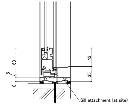
<Multi lock bottom detail>
