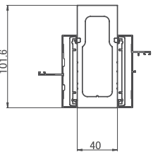
<Mullion (Large)>
