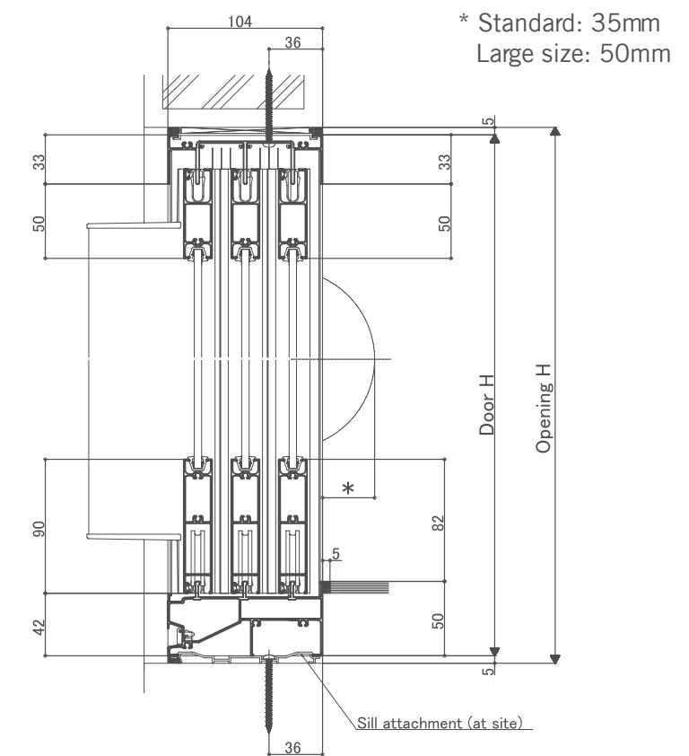
<Vertical section: 3 panels sliding door>
