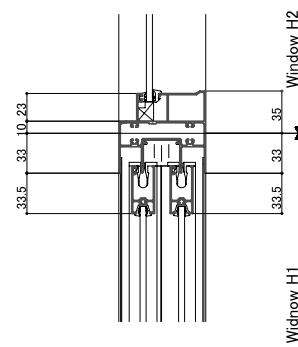
<Vertical section: Fix/Sliding transom>
