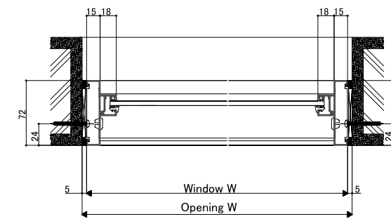
<Horizontal section: Single fix window>
