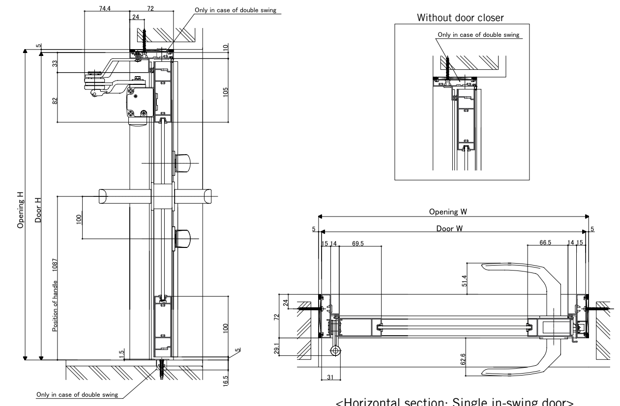
<Vertical section: Single & double in-swing door>
