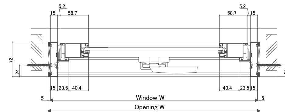
<Horizontal section: Awning (single lock)>
