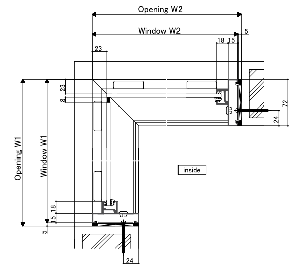
<Horizontal section: Outward fix window>
