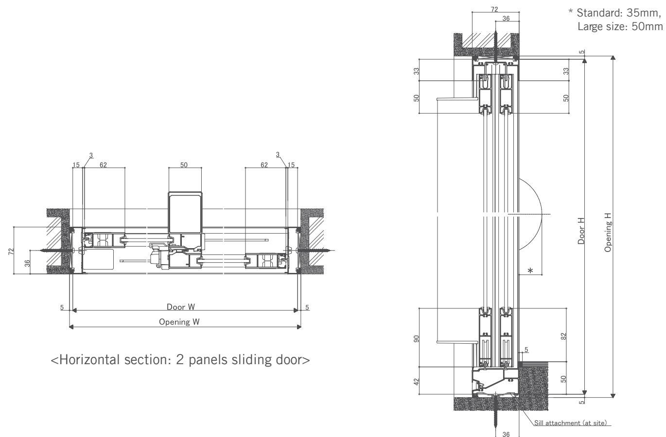
<Vertical section: 2 and 4 panels sliding door>
