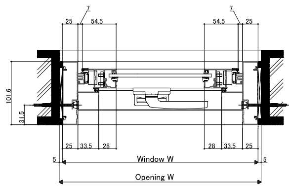
<Horizontal section: Awning window>
