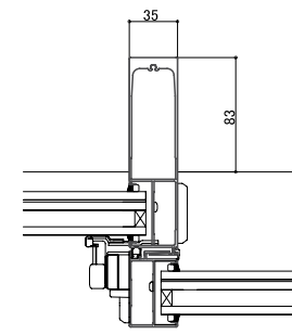
<Stile detail: In case of larger openings >
