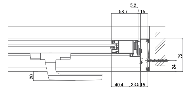
<Multi lock jamb detail>
