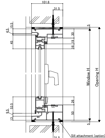
<Vertical section: Casement window>
