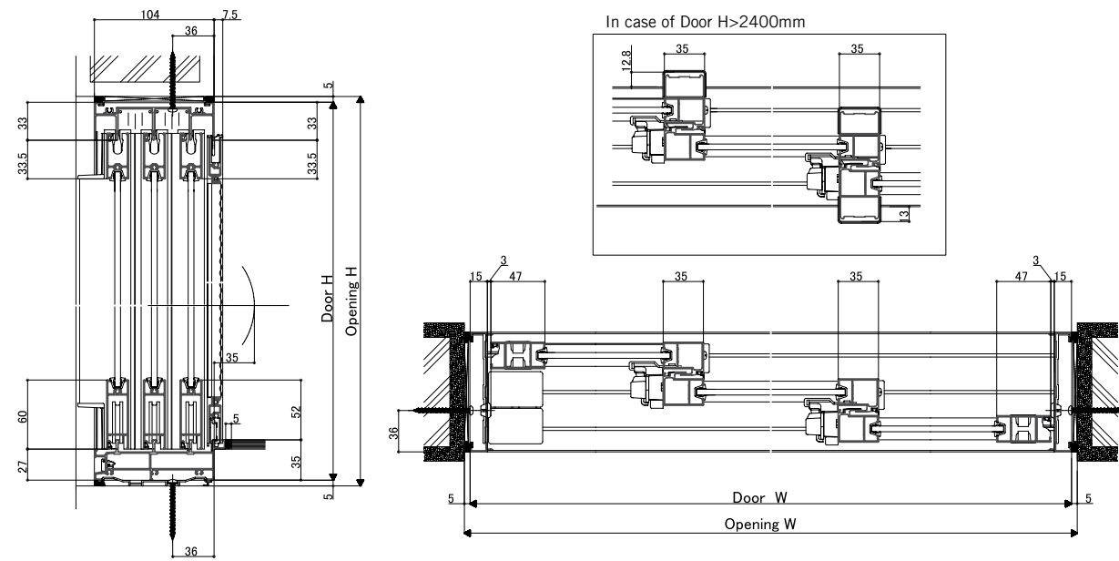
<Vertical section: 3 and 6 panels partition door>
