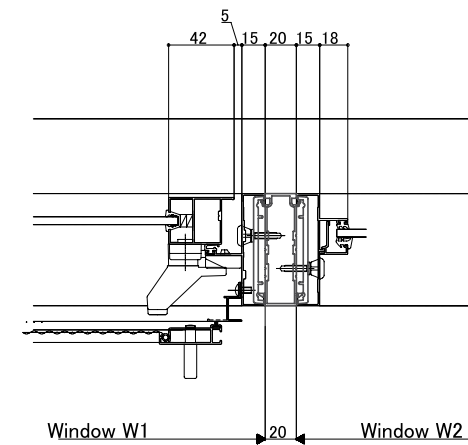
<Mullion>
