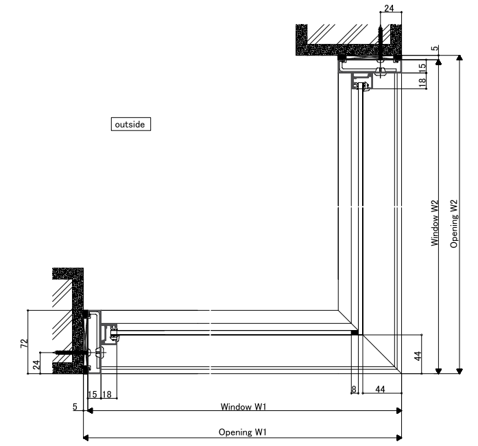
<Horizontal section: Inward fix window>
