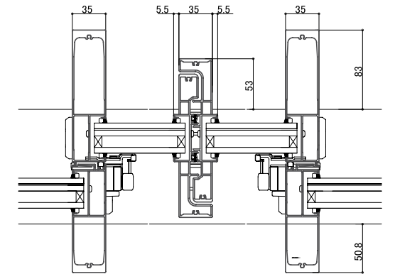
<Stile detail: In case of largest openings >
