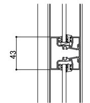
<Vertical section: With middle bar>
