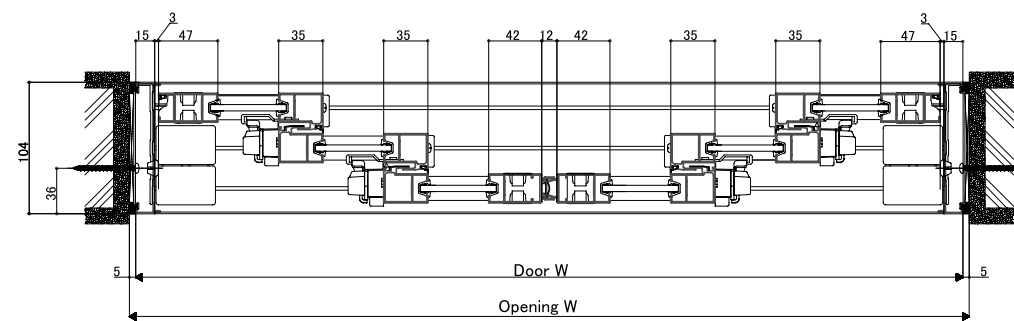
<Horizontal section: 6 panels partition door>
