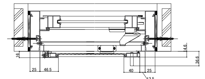
<Horizontal section: Casement with screen>
