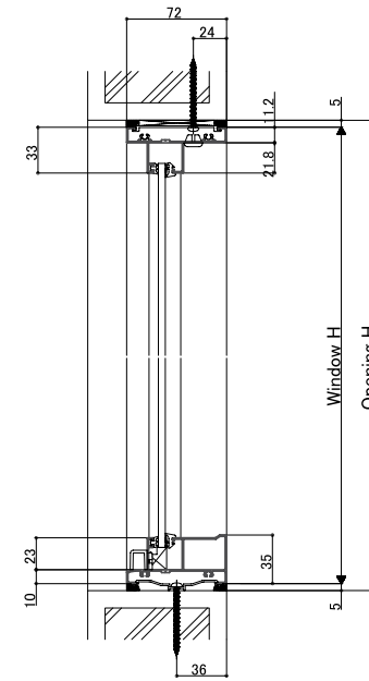
<Vertical section: Single and corner fix window>
