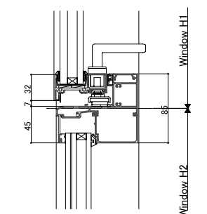
<Vertical: Projection/Fix transom>
