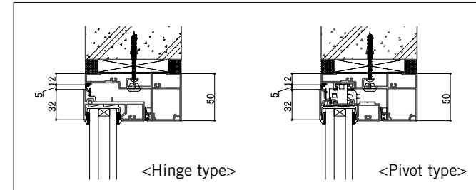
<Head detail>
