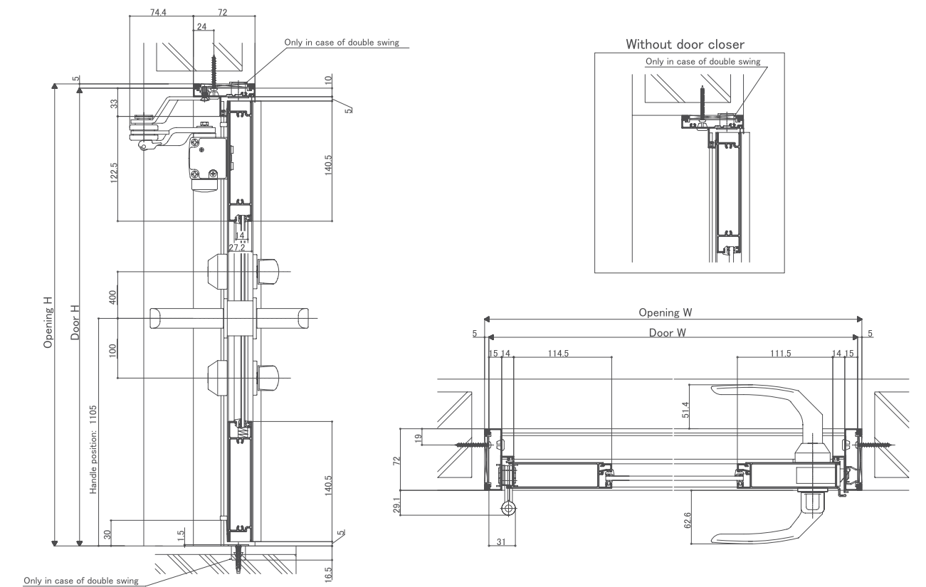
<Vertical section: Single & double in-swing door>
