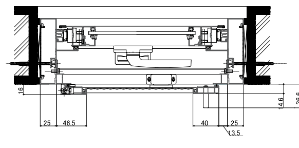
<Horizontal section: Awning with screen>
