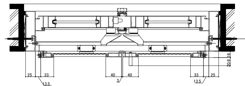
<Horizontal section: Double casement with screen>
