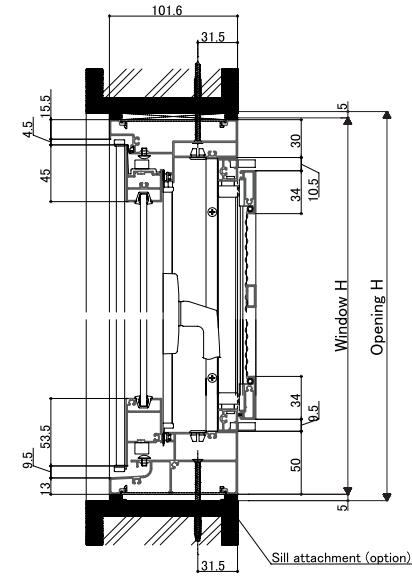
<Vertical section: Double casement with screen>
