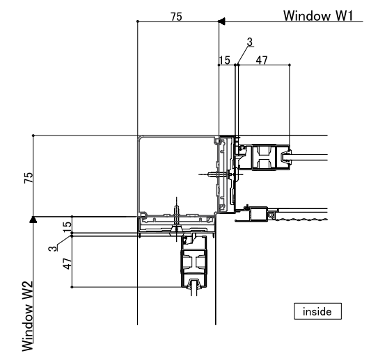
<Cor ner mullion>
