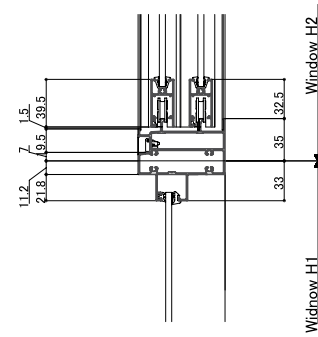
<Vertical section: Sliding/Fix transom>
