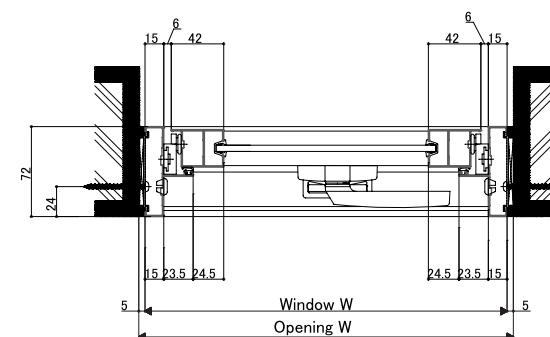
<Horizontal section: Awning window >
