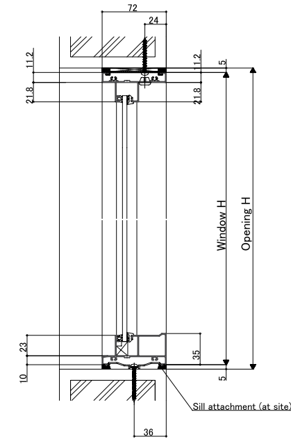
<Vertical section: Single and corner fix window>
