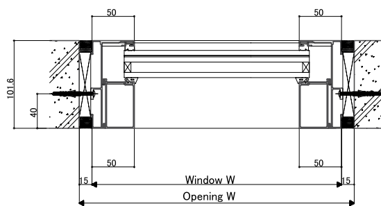
<Horizontal section: Fix window>
