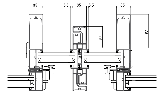
<Stile detail: In case of larger openings >
