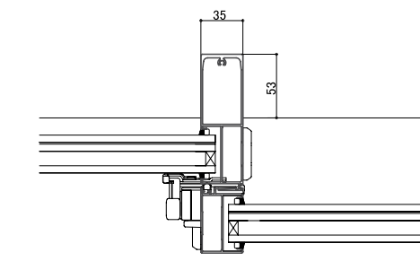
<Stile detail: In case of larger openings>
