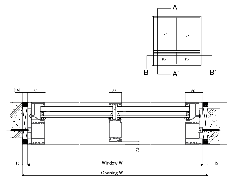
<Horizontal section: Sliding/Fix B-B'>
