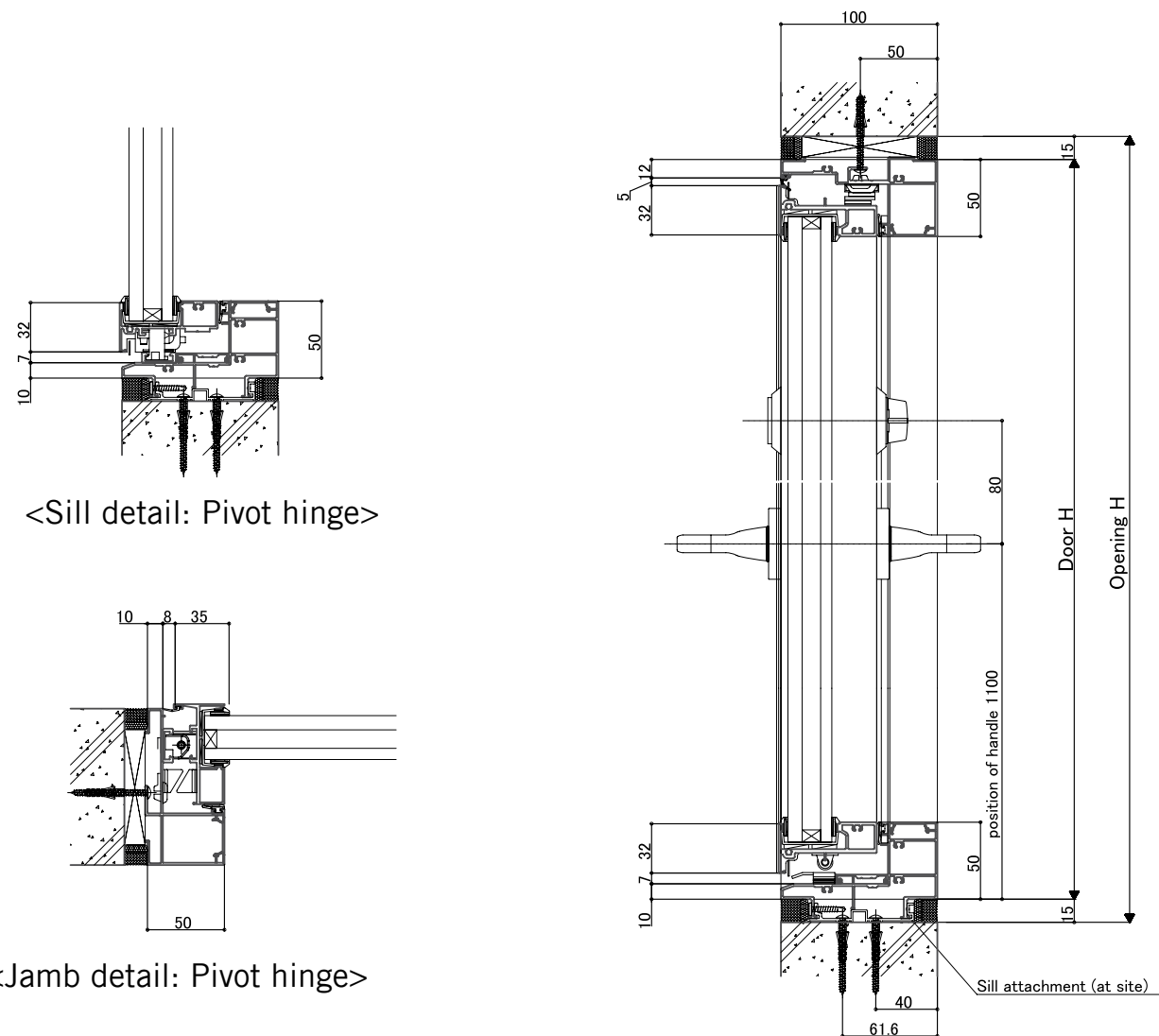
<Vertical section: Single out-swing door>
