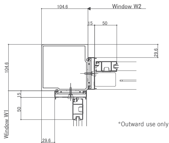
<Corner mullion (Large)>
