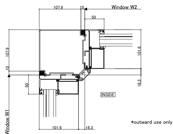
<Corner mullion>
