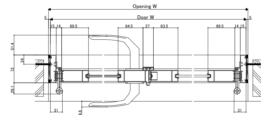
<Horizontal section: Double in-swing door>
