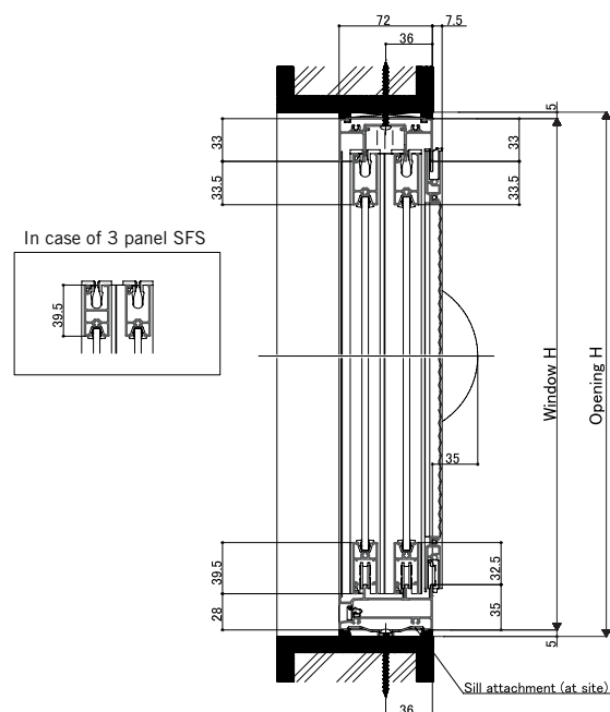
<Vertical section: 2, 4 and SFS 3 panels sliding window>
