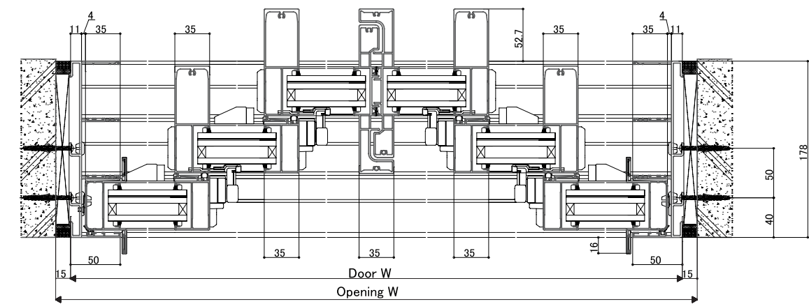
<Horizontal section: 6 panels sliding door>
