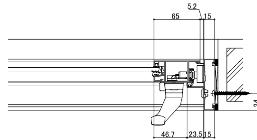
<Multi lock jamb detail>
