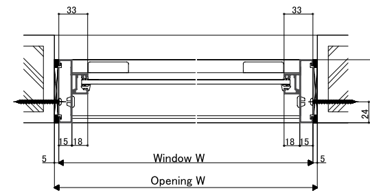
<Horizontal section: Single fix window>
