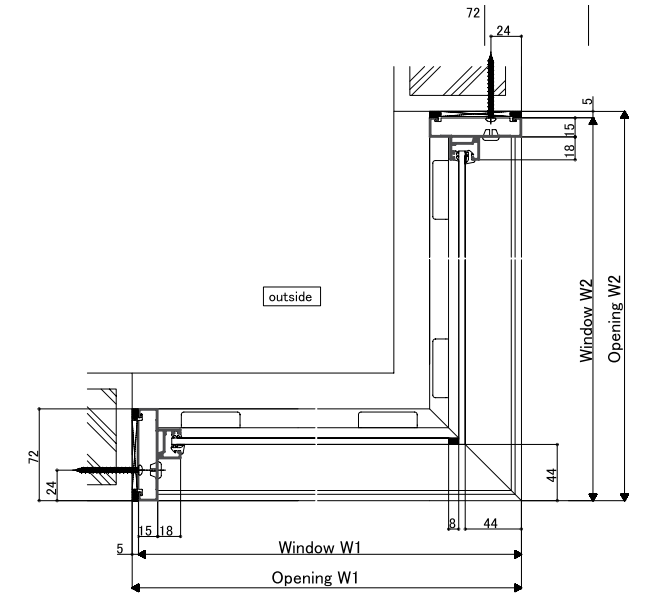
<Horizontal section: Inward fix window>
