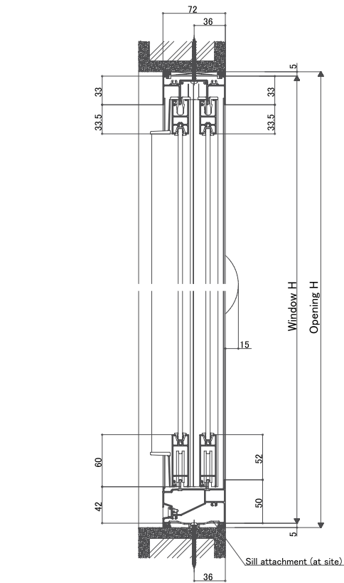
<Vertical section: 2 and 4 panels sliding window>
