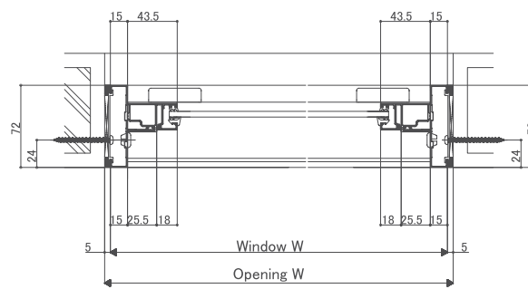
<Horizontal section window> : Combination fix
