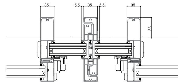
<Stile detail: In case of large openings >
