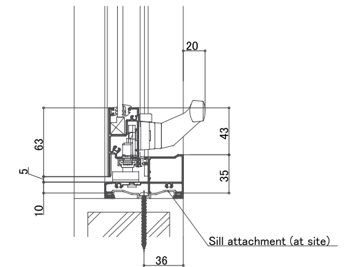
<Multi lock bottom detail>
