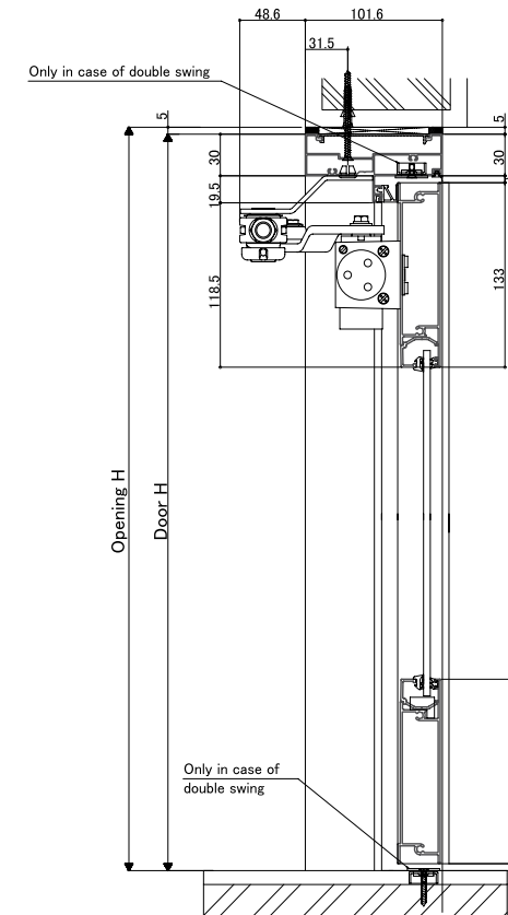
<Vertical section: Single & double in-swing door>
