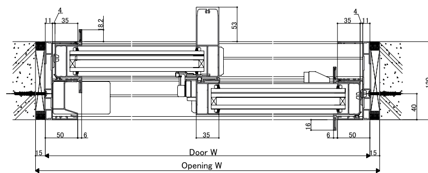
<Horizontal section: 2 panels sliding door>
