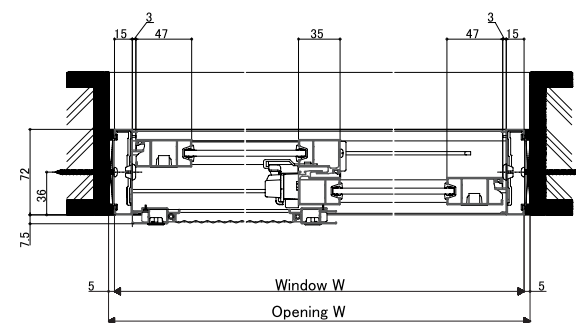
<Horizontal section: 2 panels sliding window>
