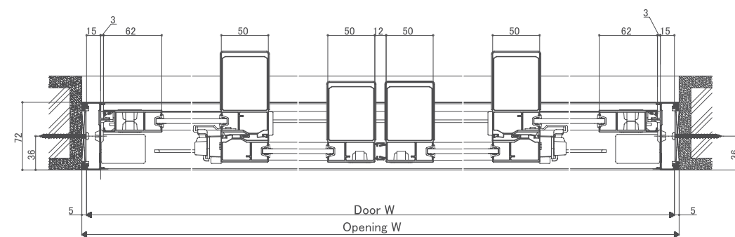
<Horizontal section: 4 panels sliding door>
