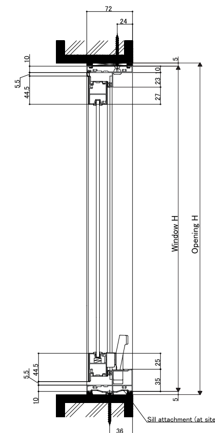
<Vertical section: Awning window>
