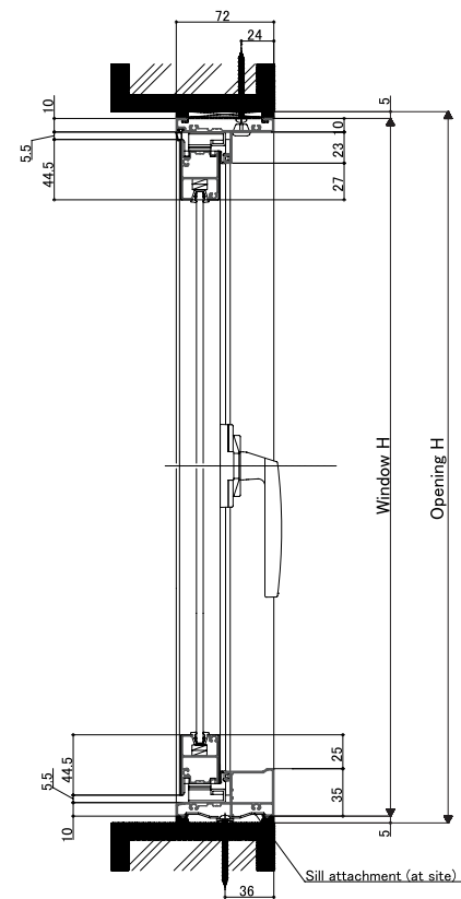
<Vertical section: Casement window>
