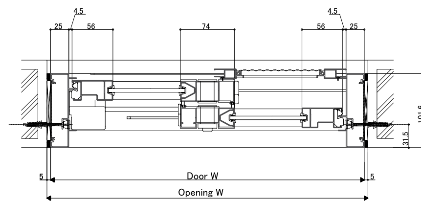
<Horizontal section: 2 panels sliding entrance door>
