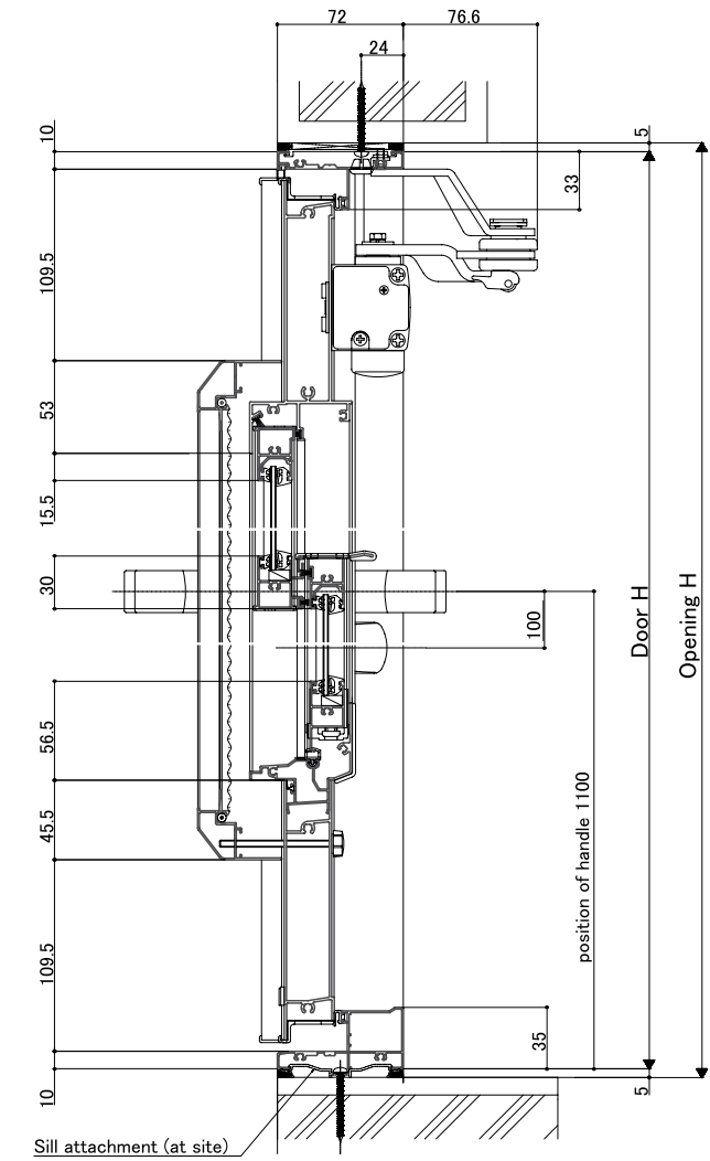
<Vertical section: Ventilation Door>
