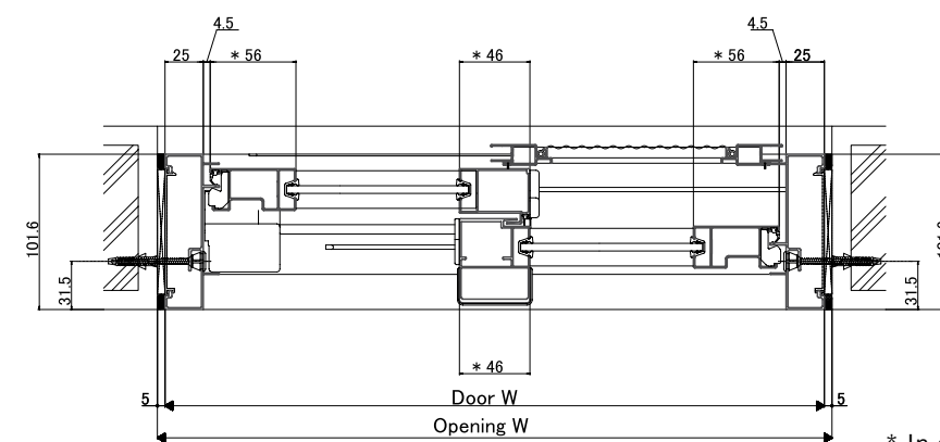
<Horizontal section: 2 panels sliding door>
