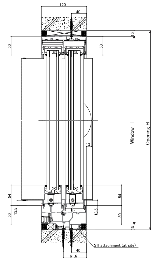
<Vertical section:4 panels sliding window >
