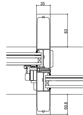
<Stile detail: In case of largest openings >
