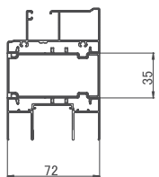
<Transom (Small)>
