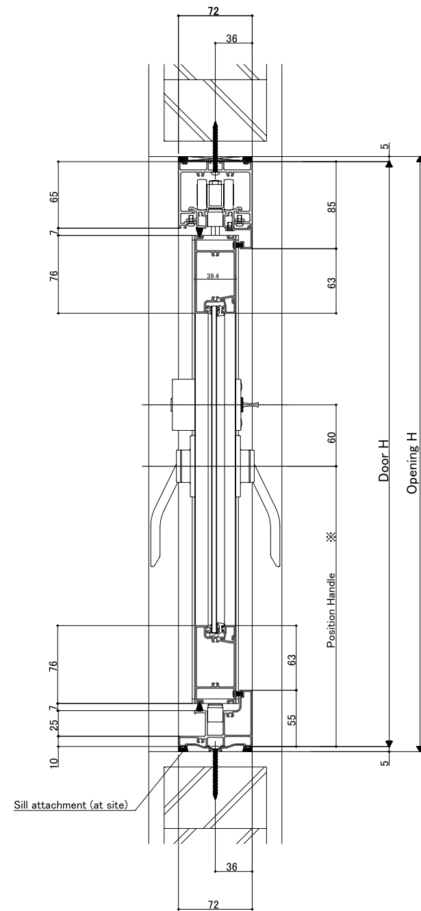
<Vertical section: Folding Door>
