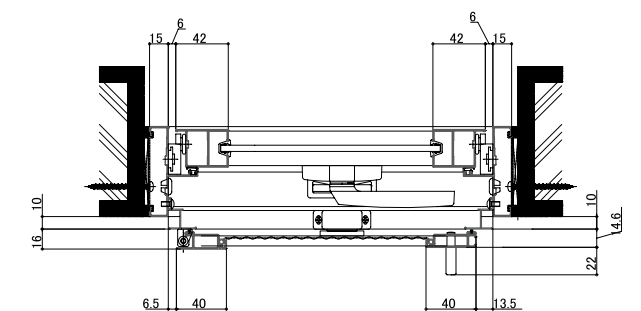
<Horizontal section: Awning with screen>
