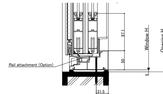
<Sill detail: With rail attachment>
