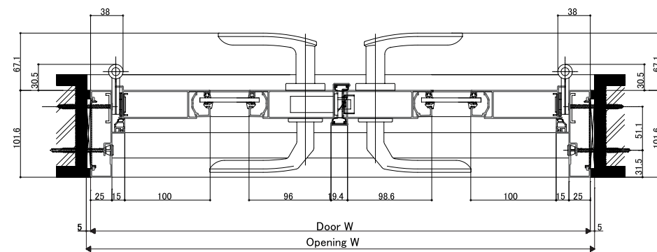
<Horizontal section: Double out-swing door>
