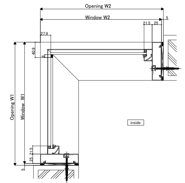
<Horizontal section: Outward fix window>
