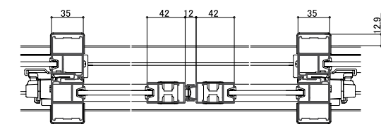
<Horizontal section: 2 panels partition door >
