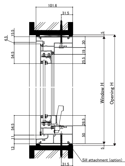
<Vertical section: Awning window>
