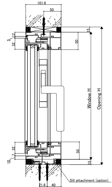
<Vertical section: Casement (with friction stay)>
