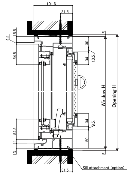
<Vertical section: Awning with screen>
